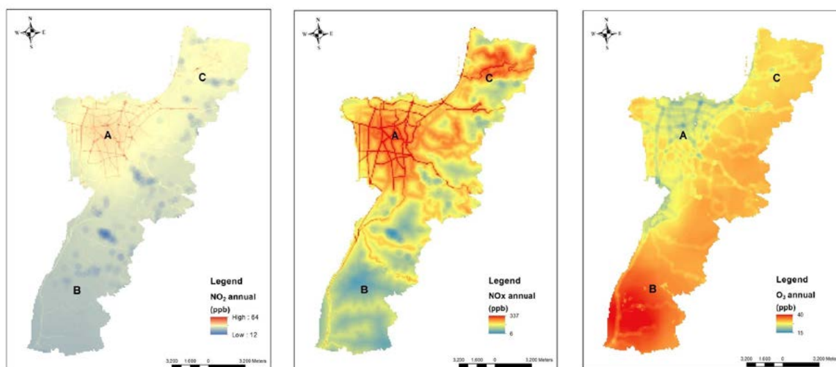
Figure 4-2 LUR Model Results for NO 2 , NO x , and O 3 Source: El Khoury, 2019
