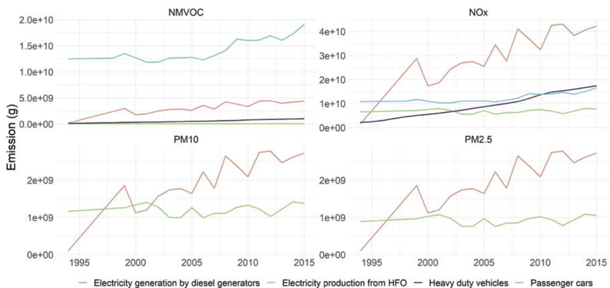
Figure 4-1 Yearly Emissions of NMVOC, NOx, \text{PM}_{2.5} and \text{PM}_{10} Note: Data was calculated using European Monitoring and Evaluation Programme 2019 emission factors. Source: Activity data for each sector is extracted from MOE/UNDP, 2019)
