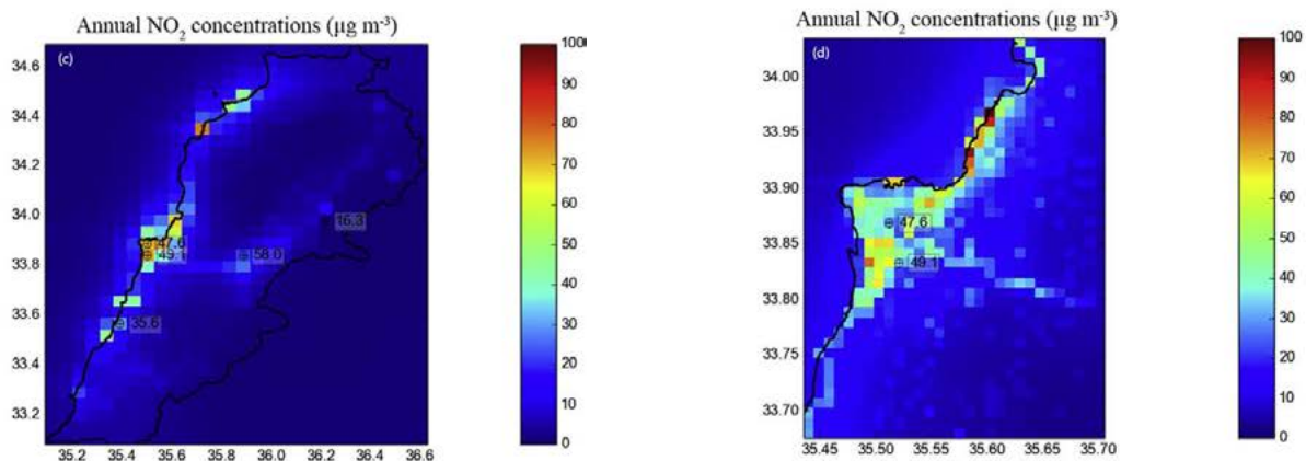
Figure 4-6 Mean Modelled Annual NO 2 Concentration Maps over Lebanon (Left) and Beirut (Right).
